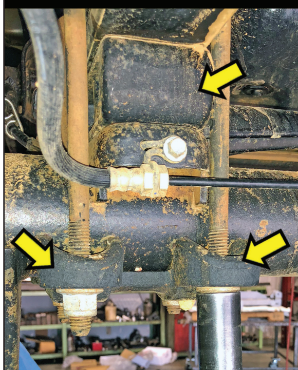
[Illustration 67] Remove Factory Rear Block.. Driver Side
